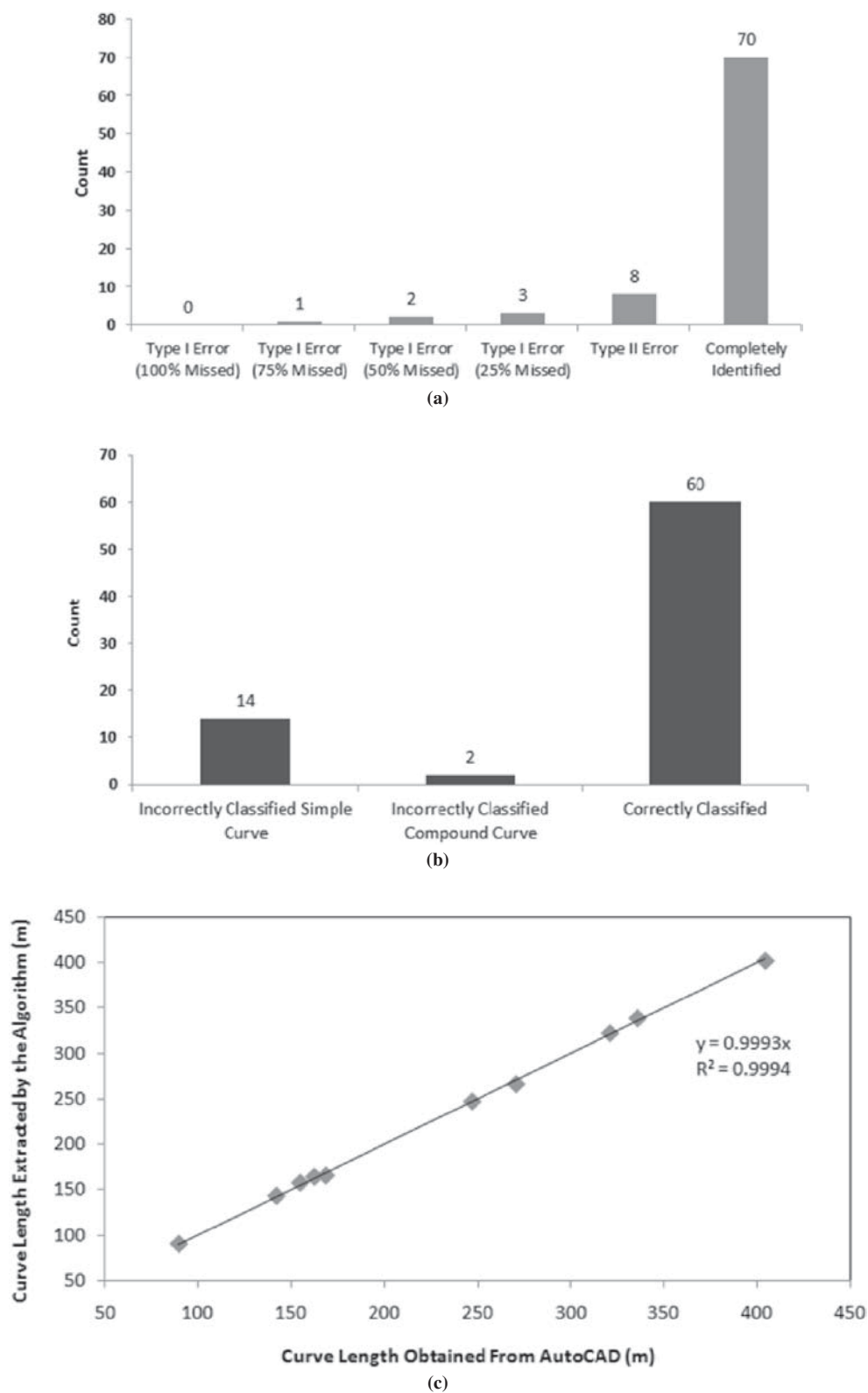
FIGURE 8 Algorithm validation results: (a) curve identification, (b) curve classification, and (c) curve length.
