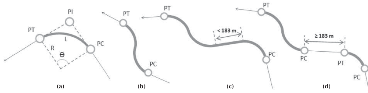
FIGURE 1 Characteristics of horizontal curves.
