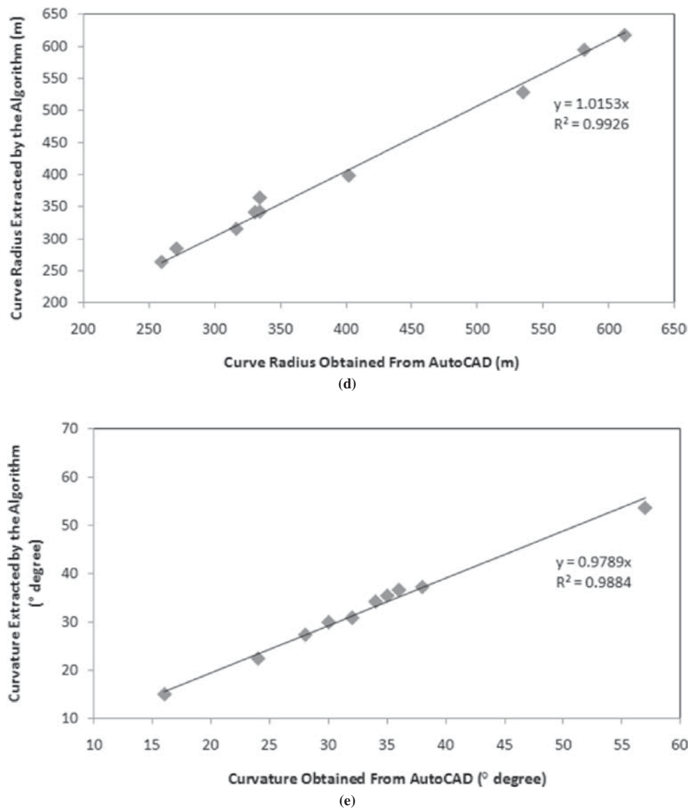
FIGURE 8 (continued) Algorithm validation results: (d) curve radius and (e) degree of curvature.
